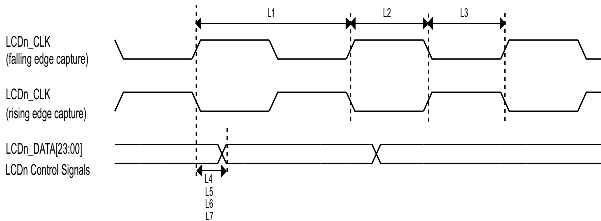
Figure 32. LCD timing
