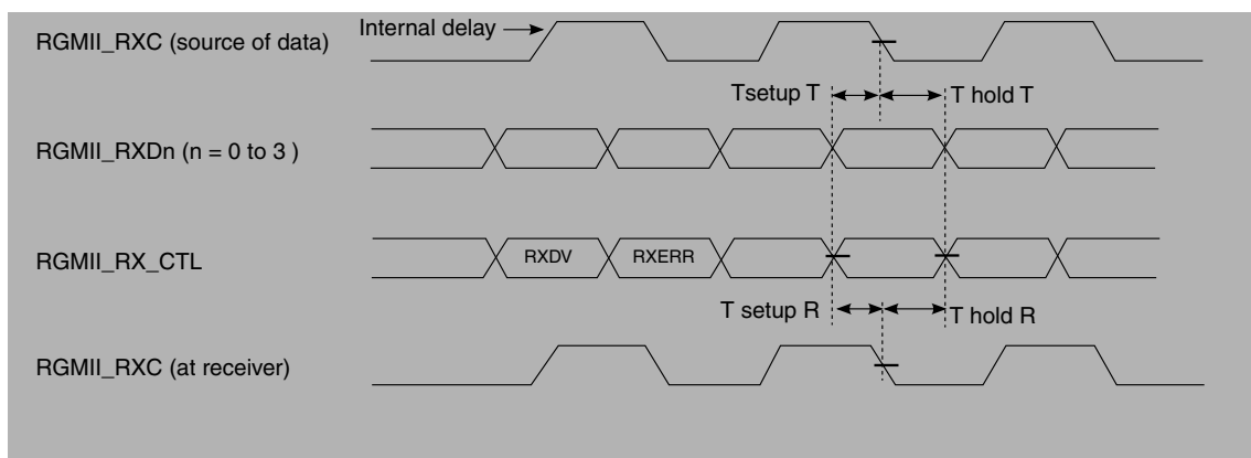
Figure 54. RGMII receive signal timing diagram with internal delay
