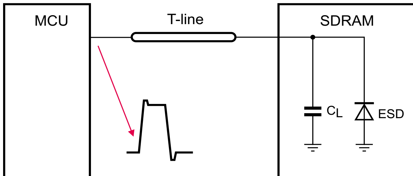
Figure 10. MCU-SDRAM circuit with overshoot/undershoot
