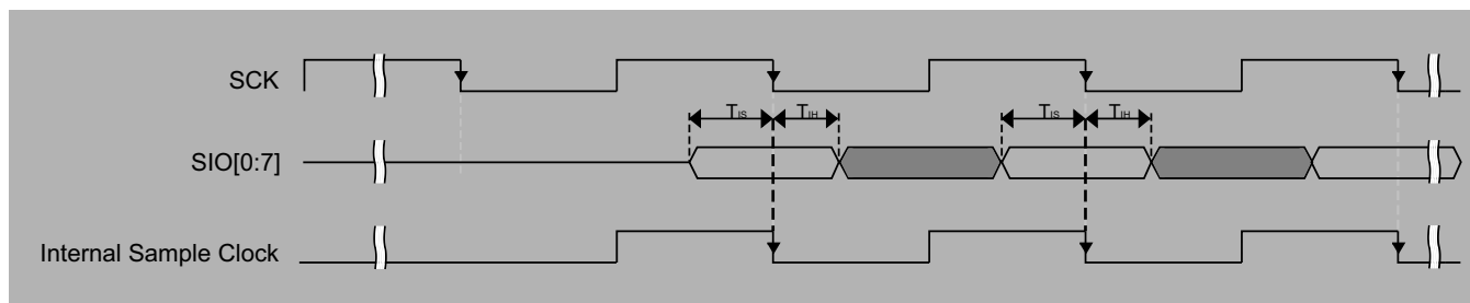
Figure 22. FlexSPI input timing in SDR mode where FlexSPI_MCR0[RXCLKSRC] = 0X0, 0X1
