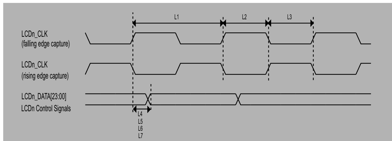
Figure 33. LCD timing
