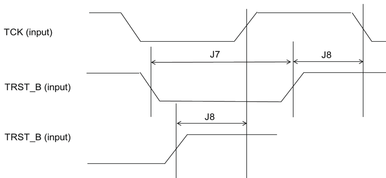
Figure 15. JTAG_TRST_B timing
