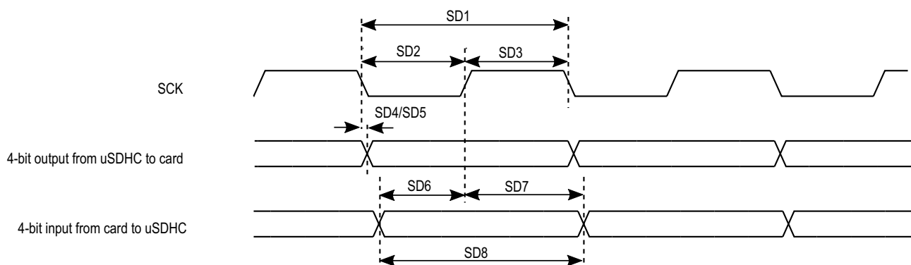
Figure 44. SDR50/SDR104 timing
