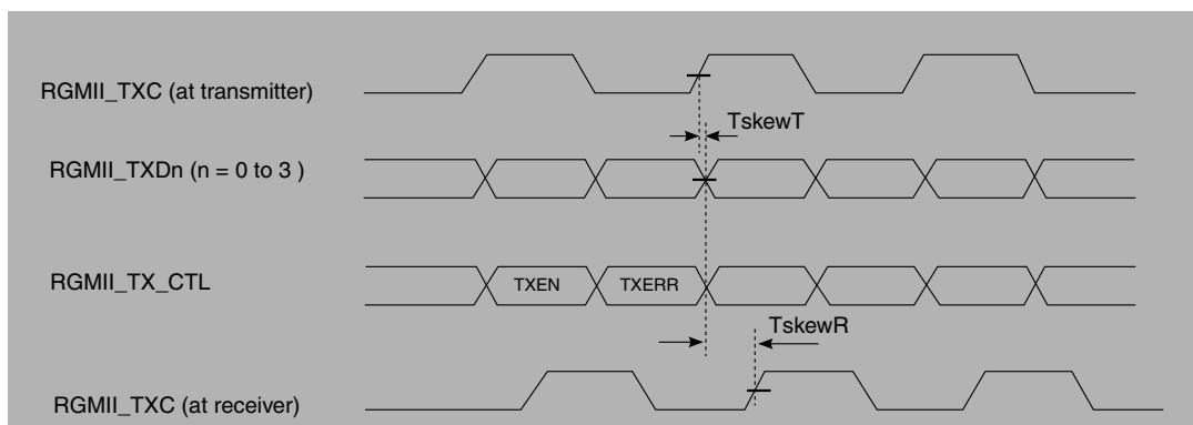
Figure 52. RGMII transmit signal timing diagram
