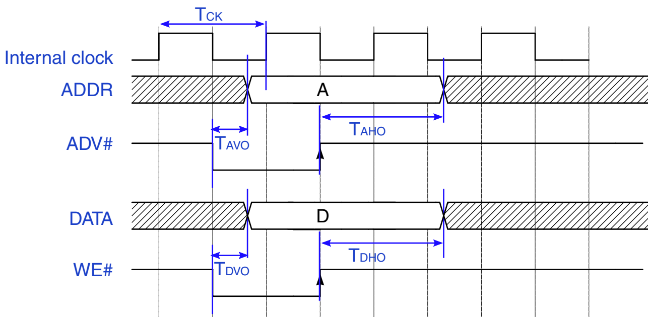
Figure 18. SEMC output timing in ASYNC mode
