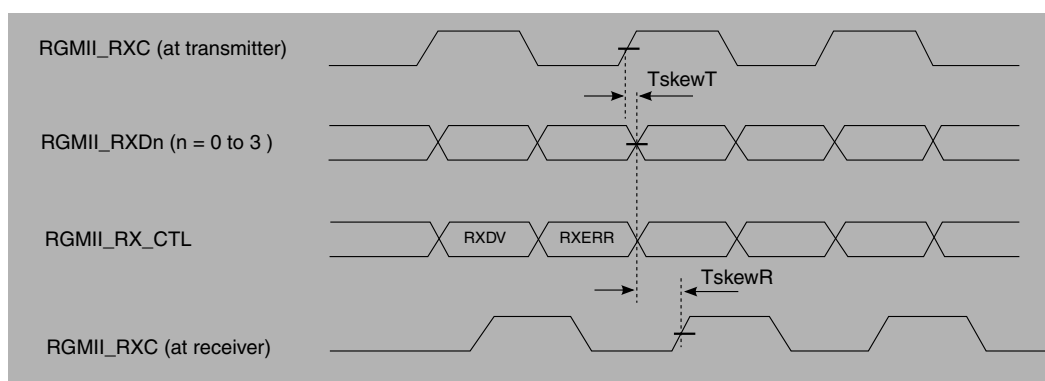
Figure 53. RGMII receive signal timing diagram
