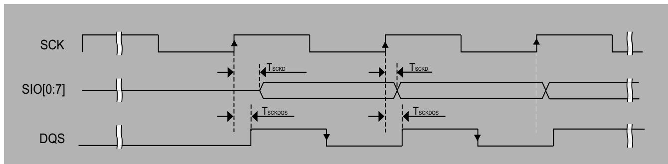
Figure 23. FlexSPI input timing in SDR mode where FlexSPI_MCR0[RXCLKSRC] = 0X3 (case A1)
