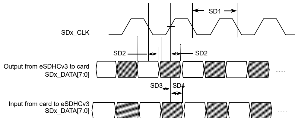
Figure 42. eMMC4.4/4.41/SD3.0 timing
