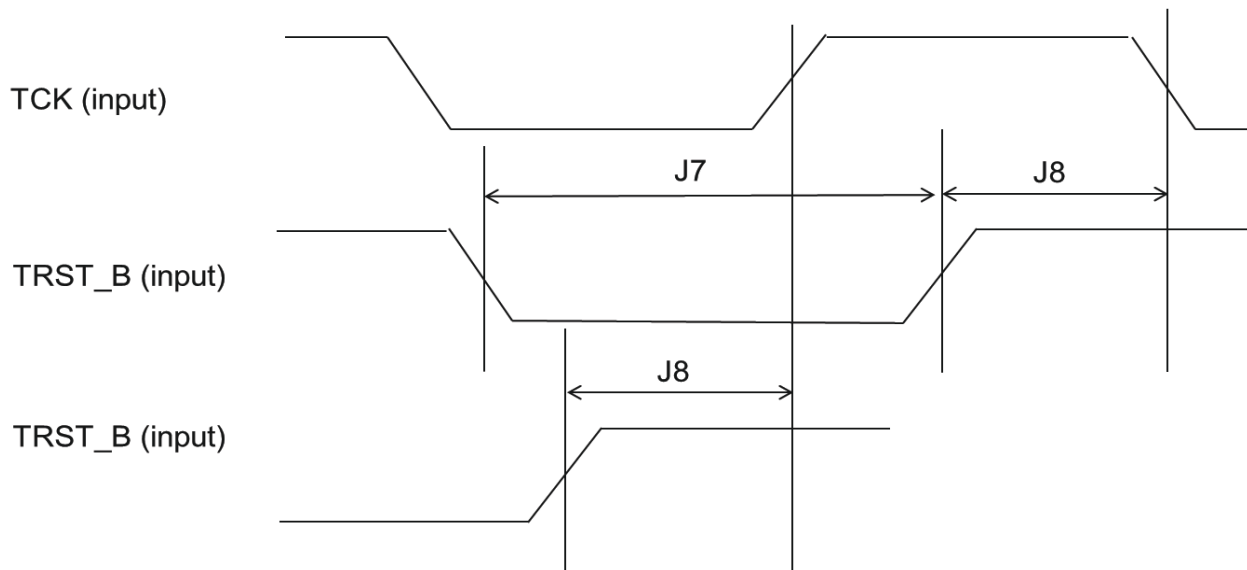
Figure 14. JTAG_TRST_B timing
