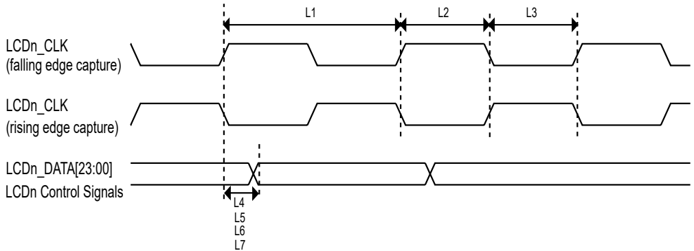
Figure 29. LCD timing
