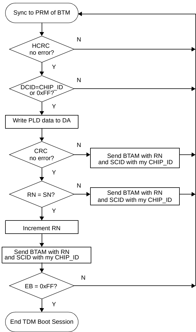
Figure 7. MSC8102 Logic Layer Protocol
