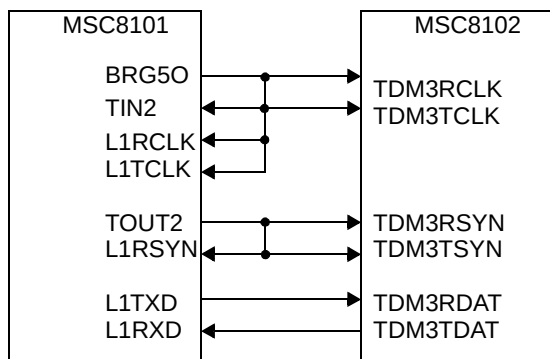
Figure 9. TDM Pin Connection
