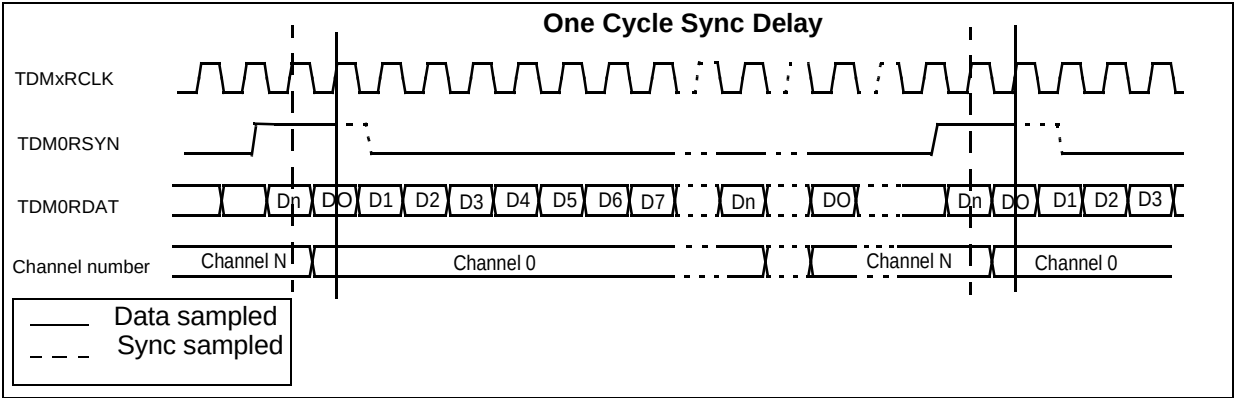
Figure 3. Receive Frame
