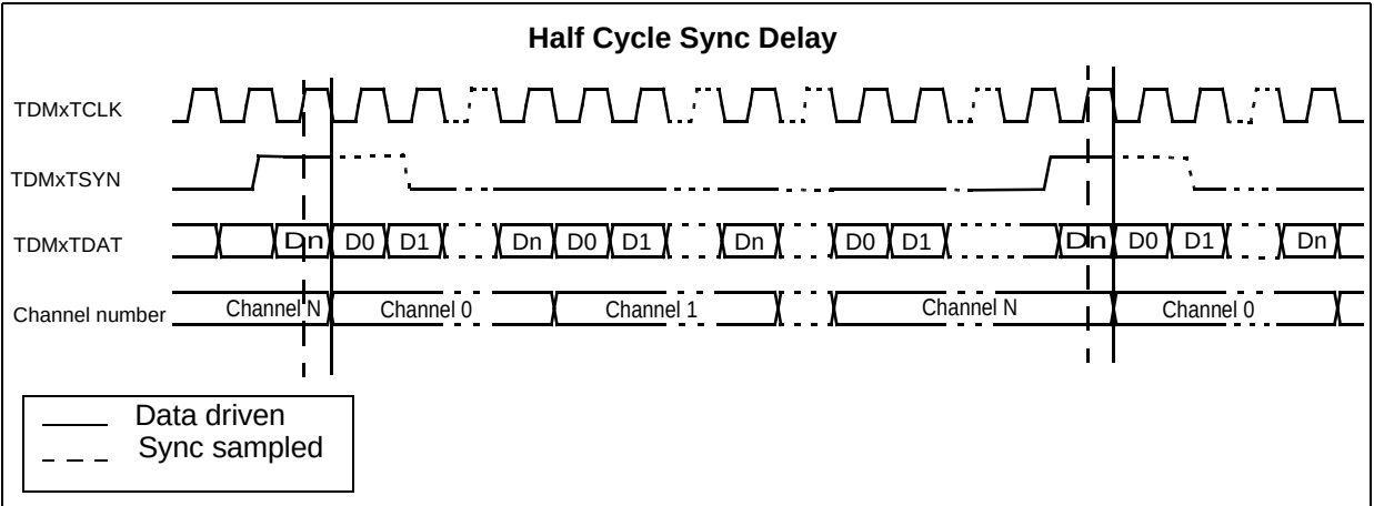
Figure 4. Transmit Frame
