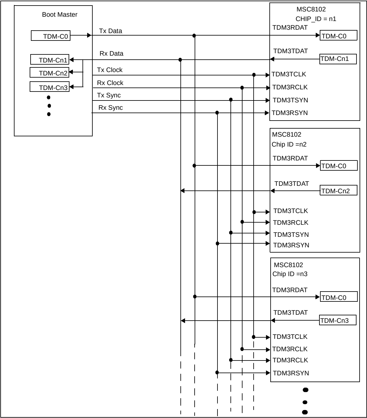
Figure 1. TDM Boot System
