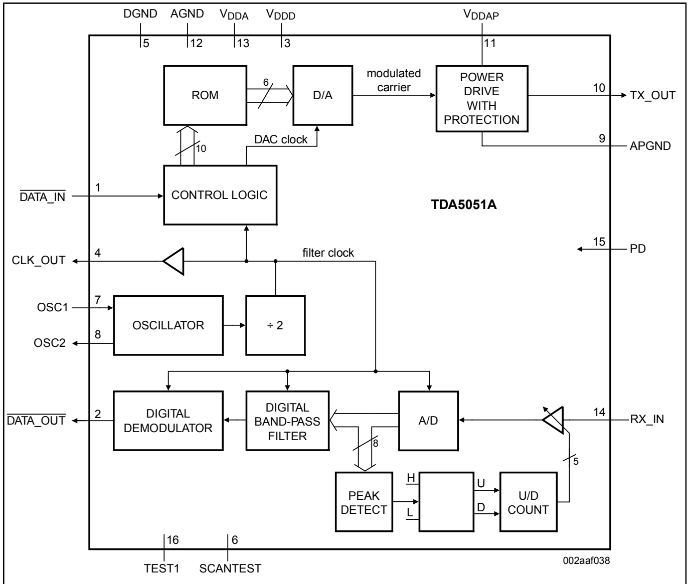
TDA5051A 框图 Block Diagram
