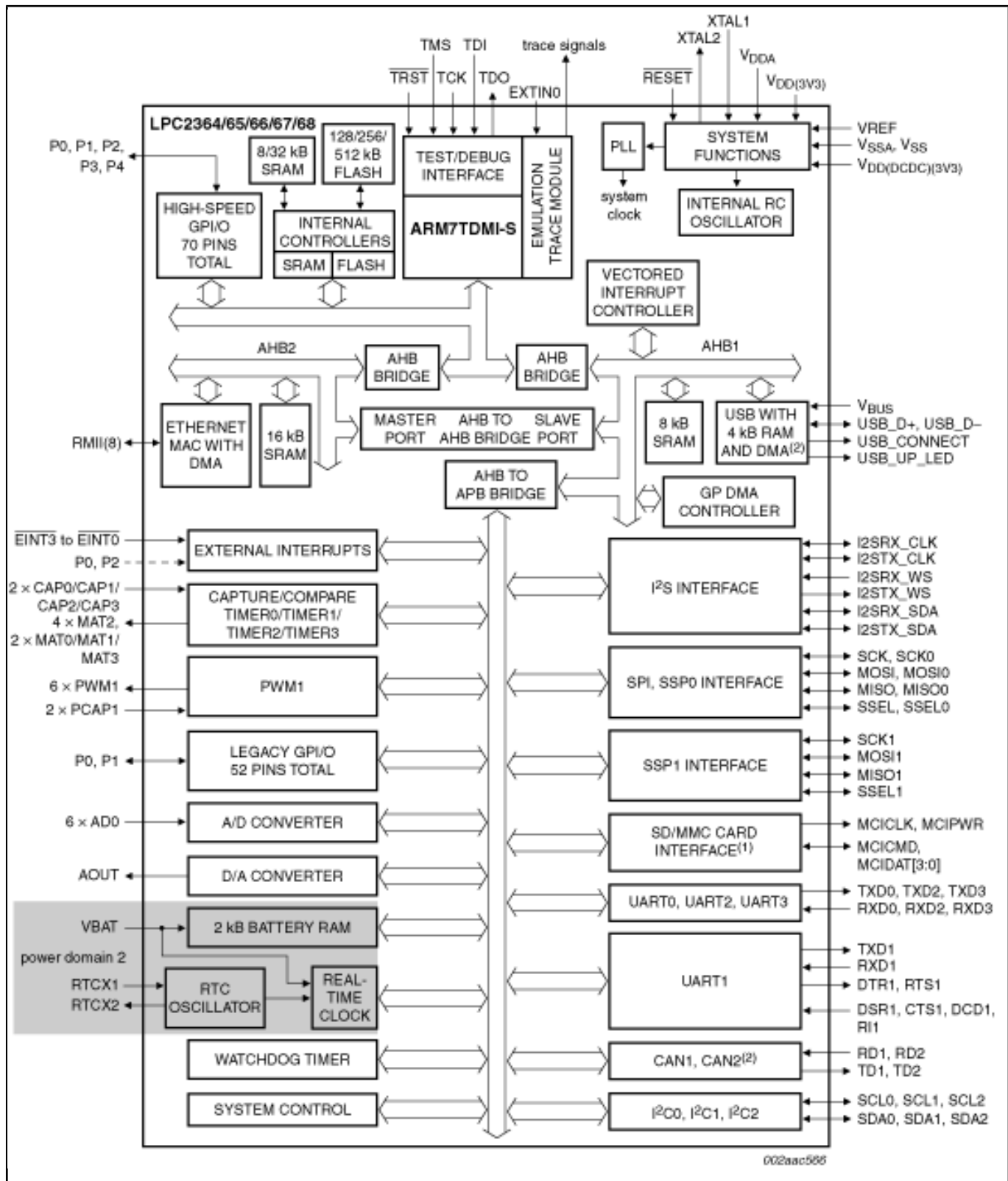
Block diagram: LPC2364FBD100, LPC2364FET100, LPC2364HBD100, LPC2365FBD100, LPC2366FBD100, LPC2367FBD100, LPC2368FBD100, LPC2368FET100 Block Diagram
