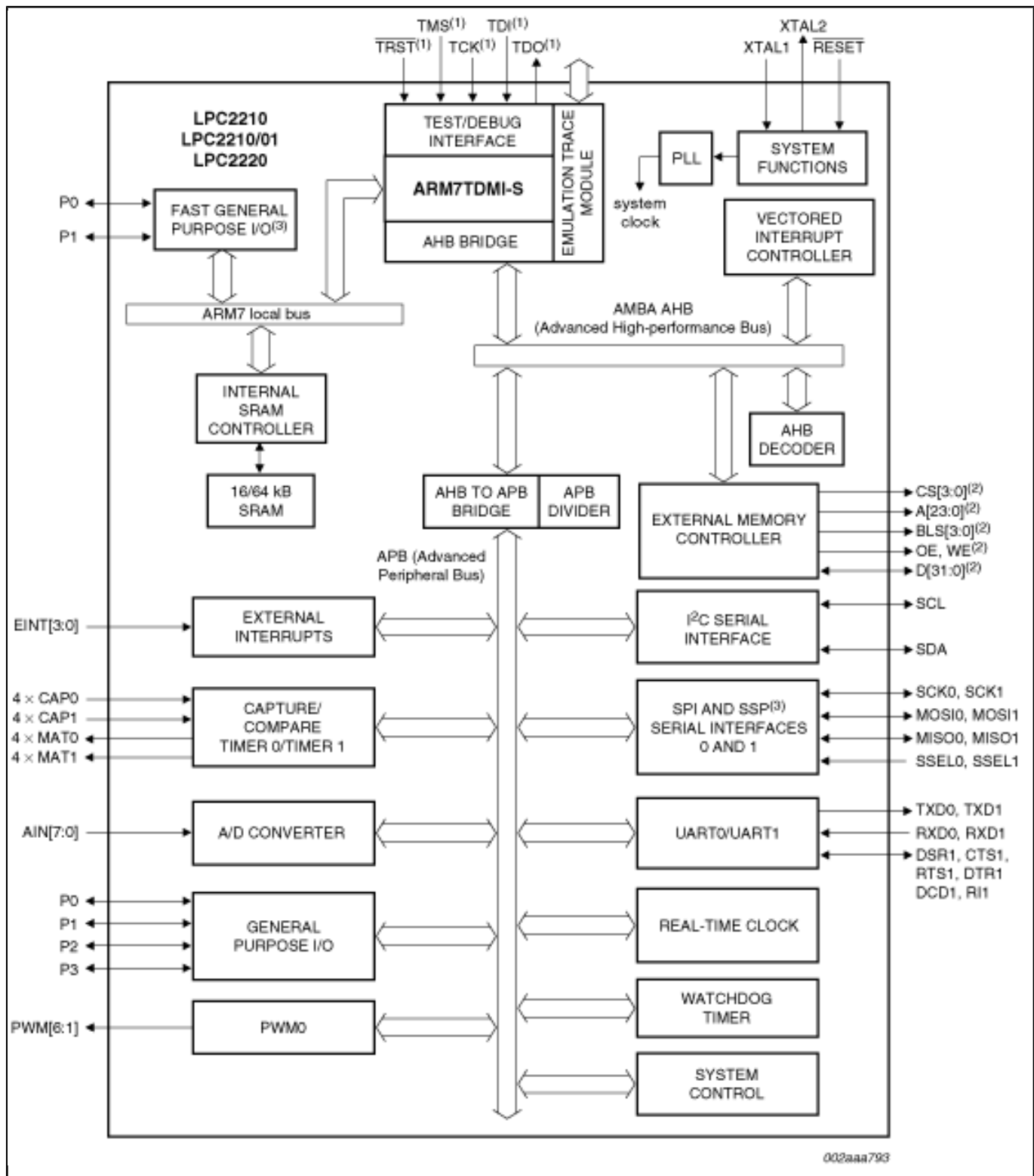
Block diagram: LPC2210FBD144, LPC2220FBD144, LPC2220FET144 Block Diagram
