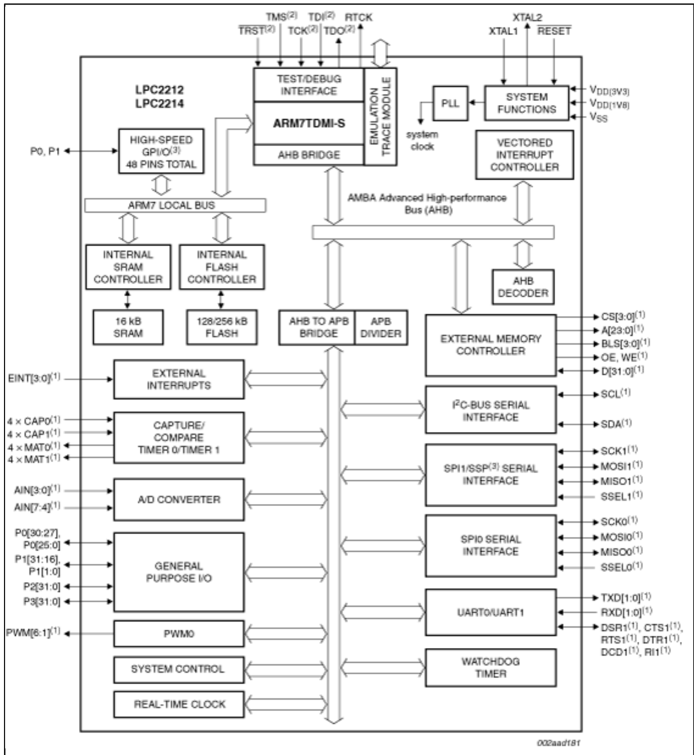
Block diagram: LPC2212FBD144, LPC2214FBD144 Block Diagram
