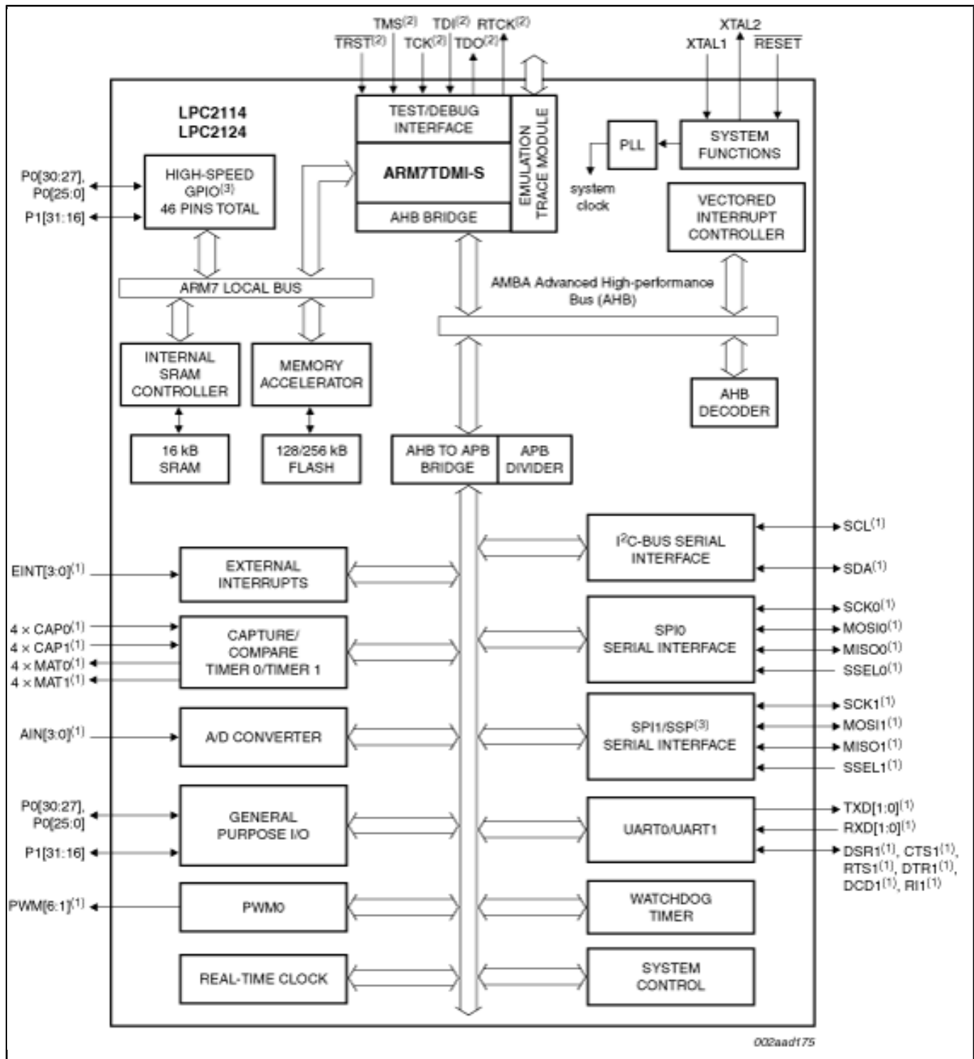
Block diagram: LPC2114FBD64, LPC2124FBD64 Block Diagram
