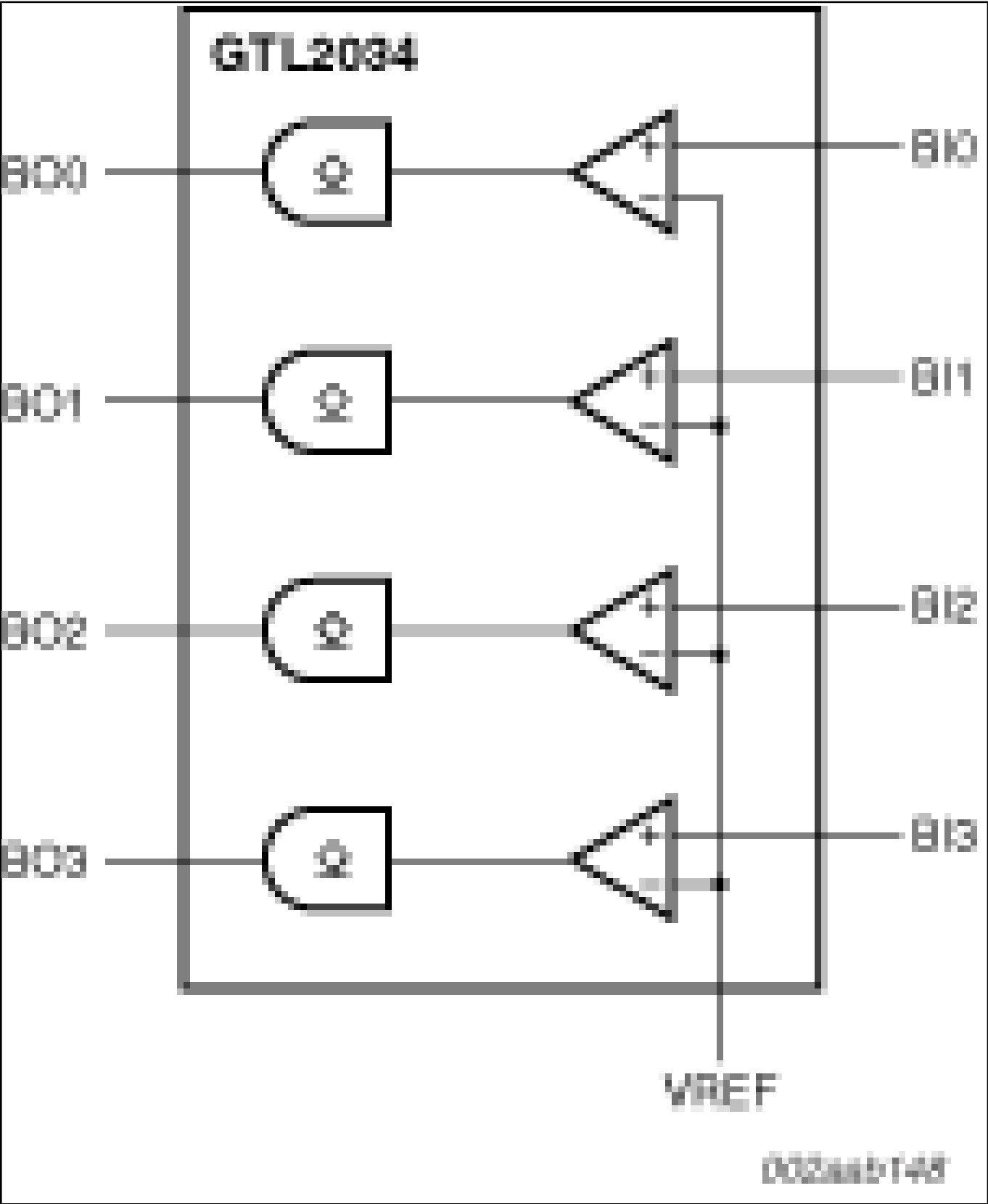
Block diagram: GTL2034PW Block Diagram
