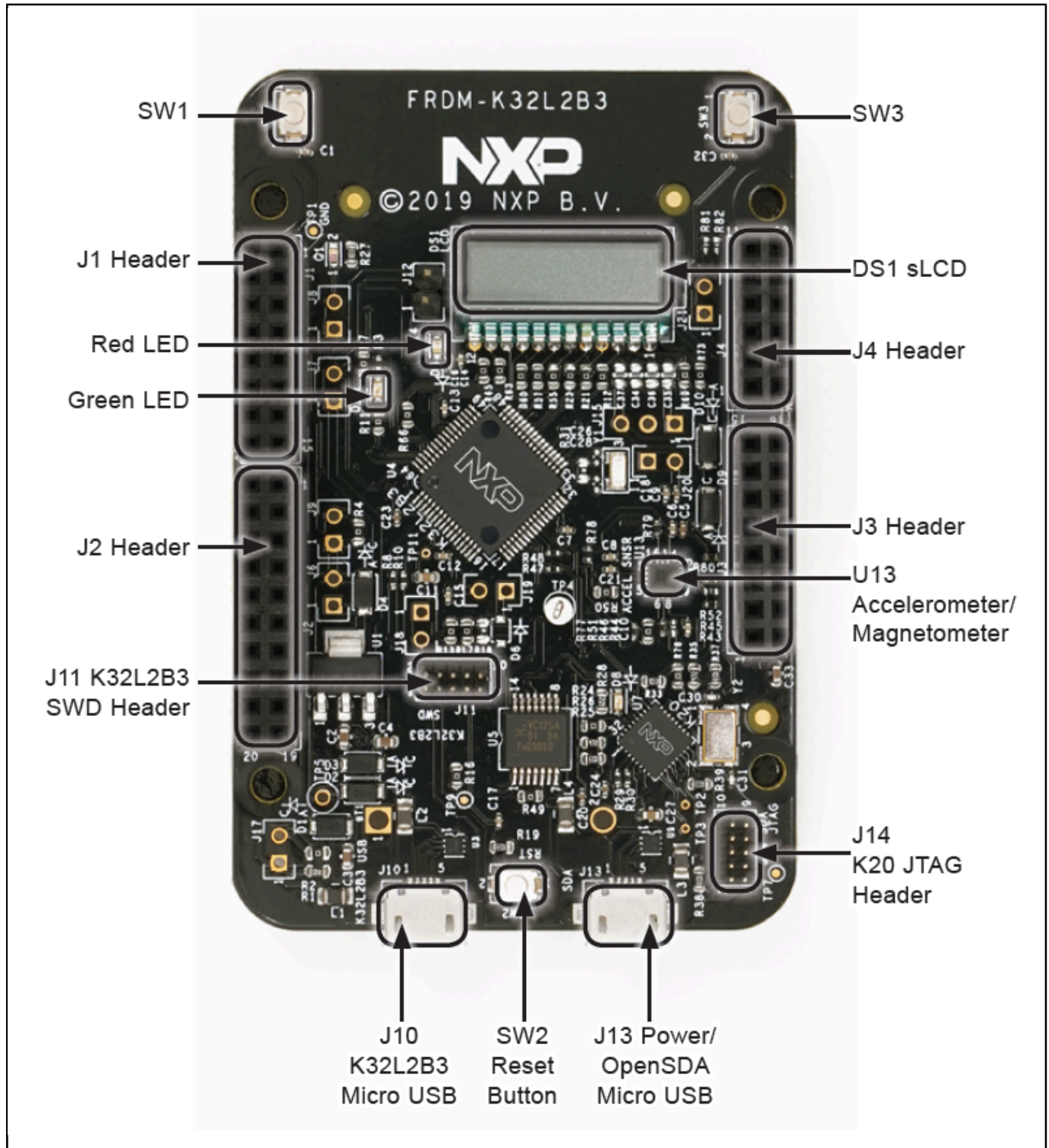
FRDM K32L2B Block Diagram
