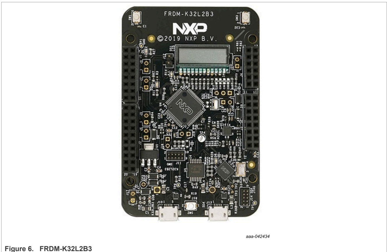
Figure 6. FRDM-K32L2B3
